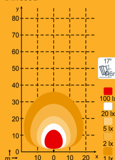
N4702 14400lm Diffused
