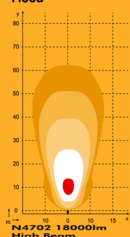
N4702 18000lm Flood
