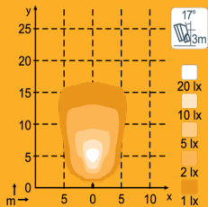
Antares Go 610 1000lm Wide Flood
