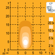
Antares Go 610 1000lm Flood
