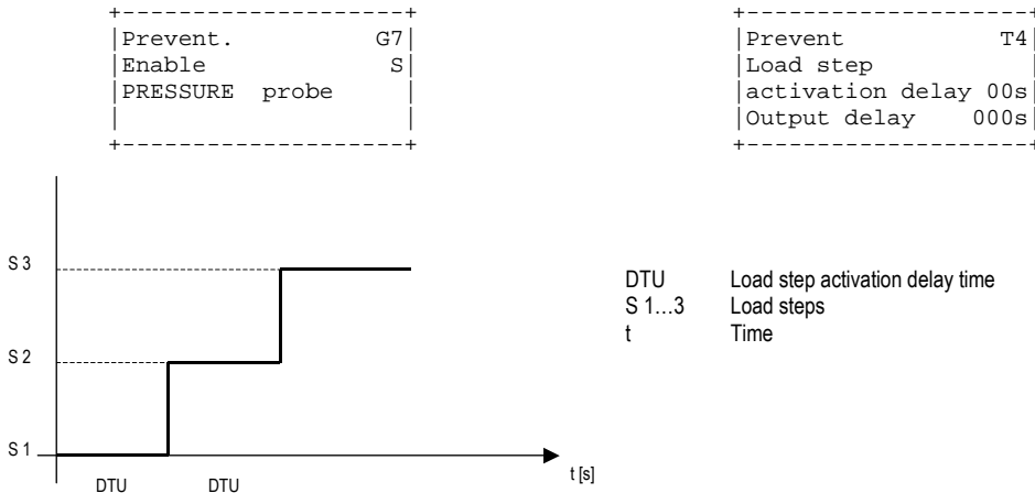
Fig. 15.2 Forcing of compressor load steps to prevent high condensing pressure
