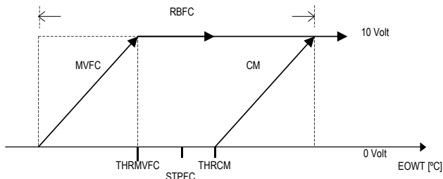
Fig. 18.12 0 to 10 V freecooling valve - proportional condenser control - proportional control
