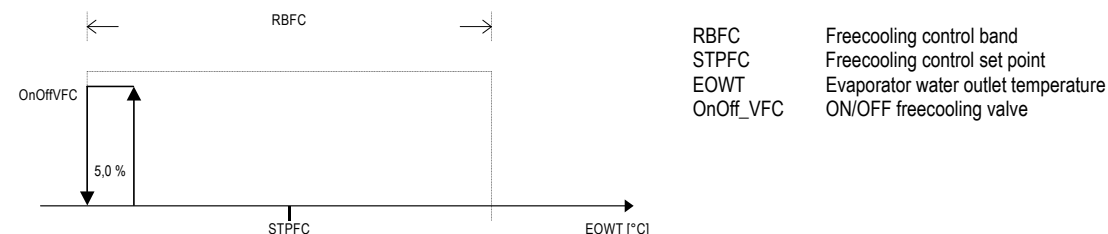
Fig. 18.4 ON/OFF freecooling valve - proportional control
