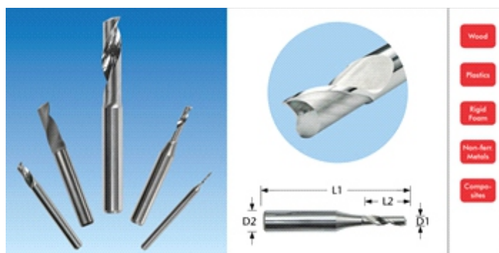
All-rounders: single tooth cutters of finest grain carbide.
