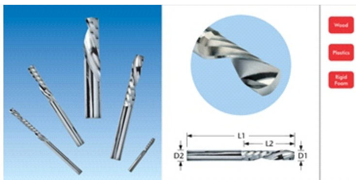
Cutters with left-hand twist for acrylic and plastics.
