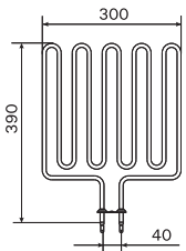
ZSK-732 1750W/240V L20
