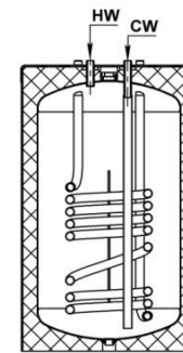
SECTION C-C
