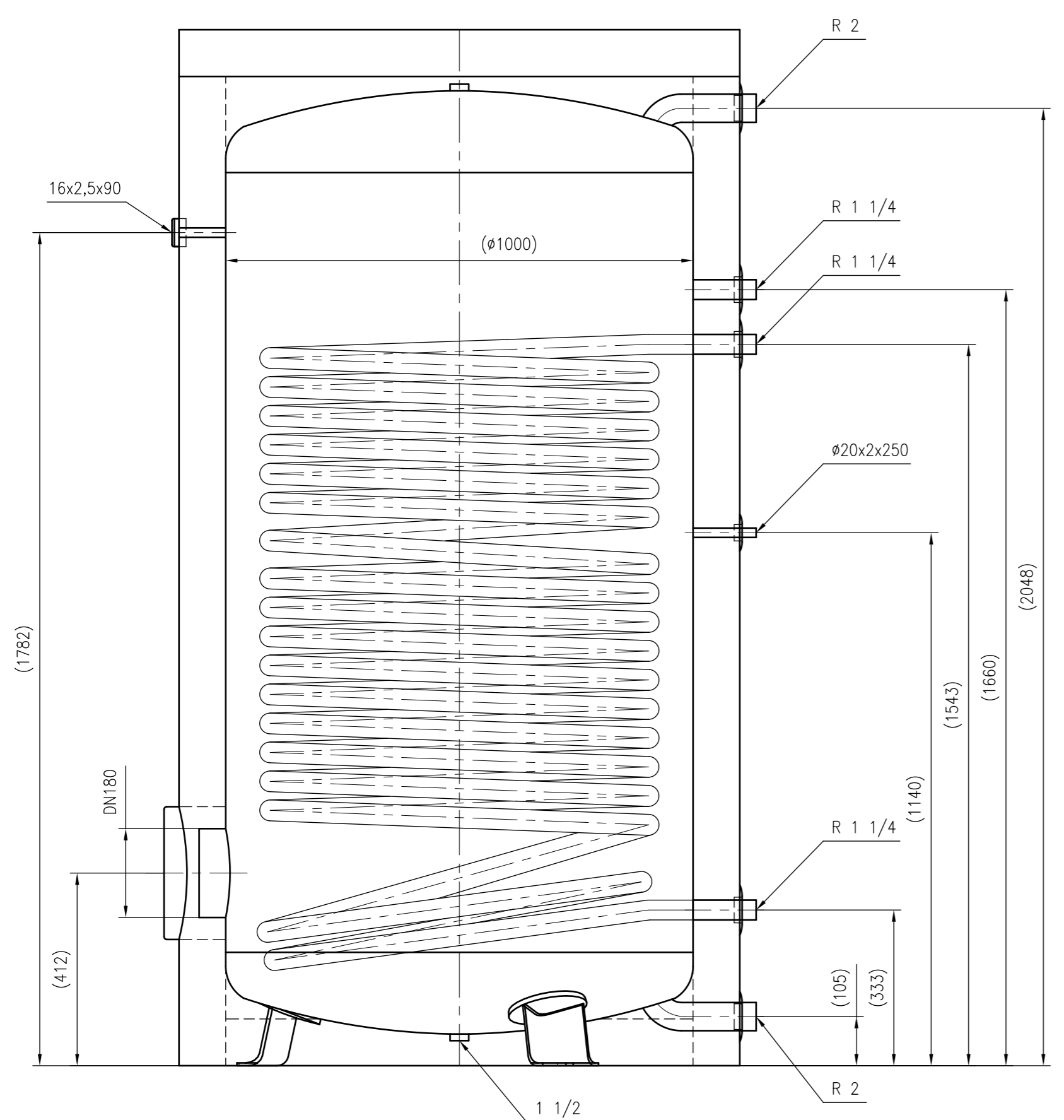
Side view
