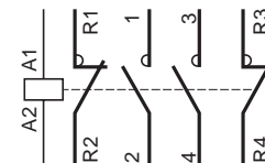
LC1E40...95008
