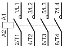
LC1E06...95004
