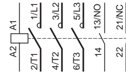
LC1E120/160
