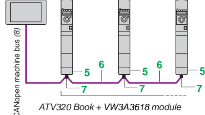
Example of connection to the CANopen machine bus via SUB-D connector
