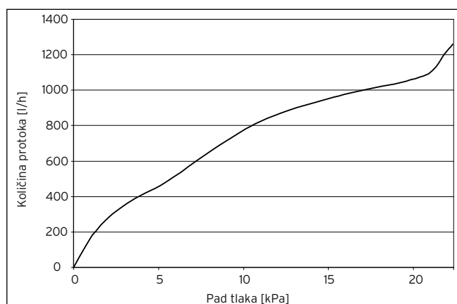
13.1 Pad tlaka eloBLOCK
